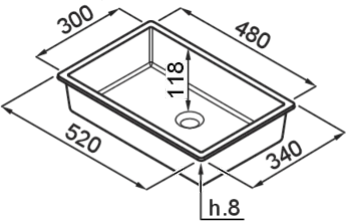
Technical Drawing
